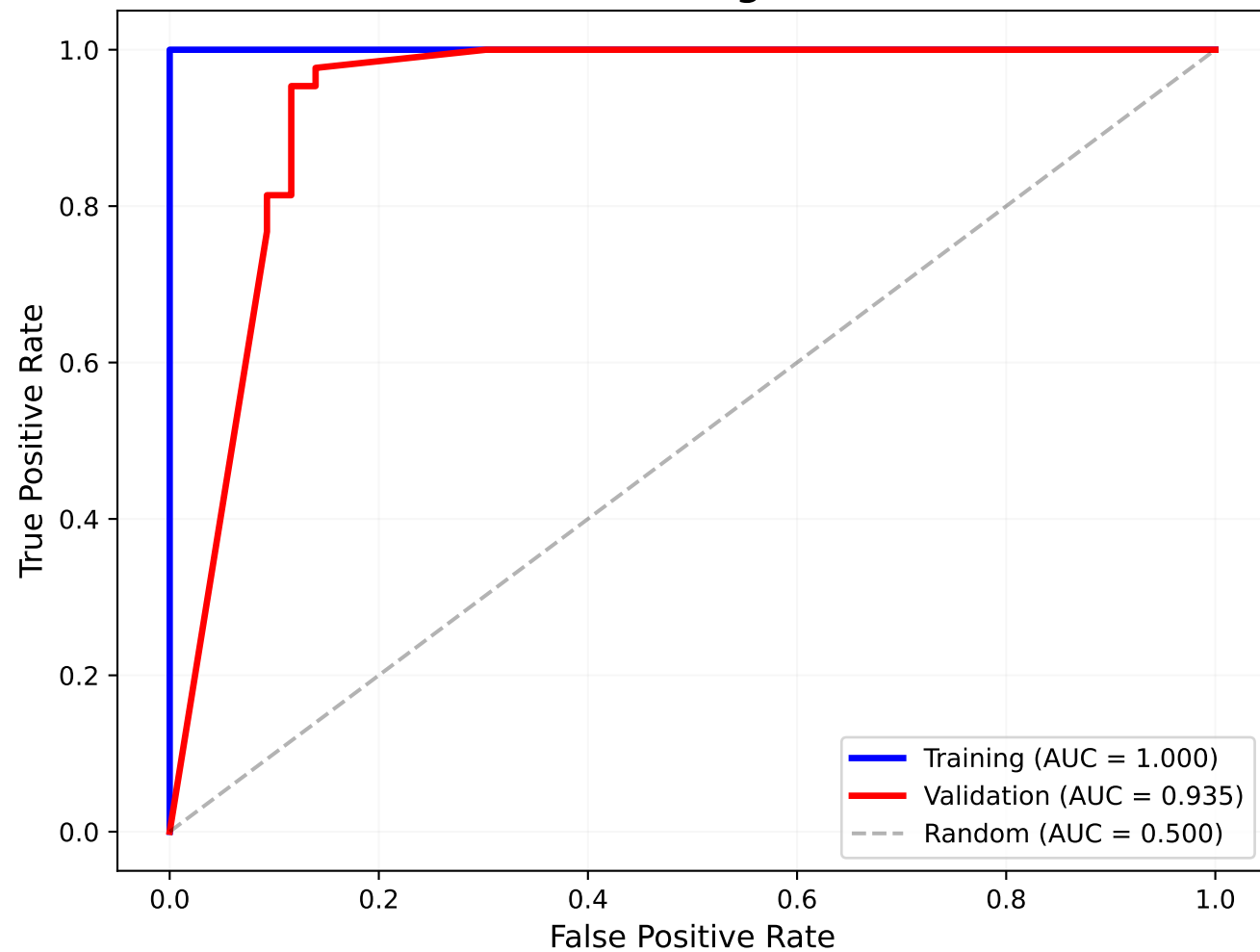
ROC Curves (Training vs Validation)
