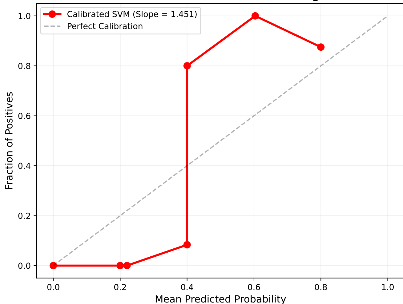
Calibration Curve (Platt Scaling)
